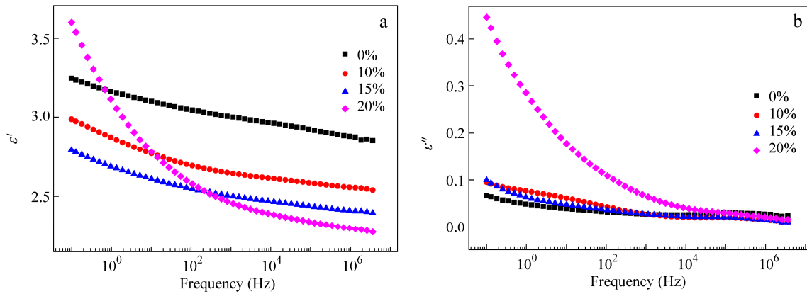
Fig. 3 Frequency dependence of real and imaginary parts ( \epsilon' and \epsilon'' ) of complex permittivity of cast films with different \text{MgAc}_2 contents
