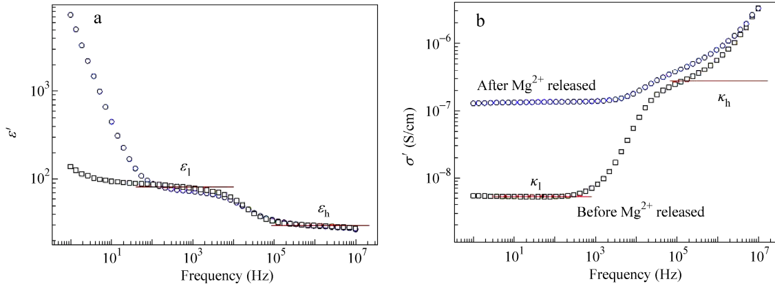
Fig. 10 Frequency dependence of real part of complex permittivity ( \epsilon' ) and conductivity ( \sigma' ) of films measured in water using liquid cell ( C_{\text{MgAc}_2} = 10 \text{ wt\%} and T_{\text{casting}} = 50 \text{ }^\circ\text{C} )
