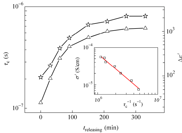
Fig. 9 Time dependence of characteristic relaxation time ( \tau_c , star) and interfacial polarization induced dielectric increment ( \Delta\epsilon' , triangle) of a film ( C_{\text{MgAc}_2} = 10 \text{ wt\%} and T_{\text{casting}} = 50 \text{ }^\circ\text{C} ) submerged in water
